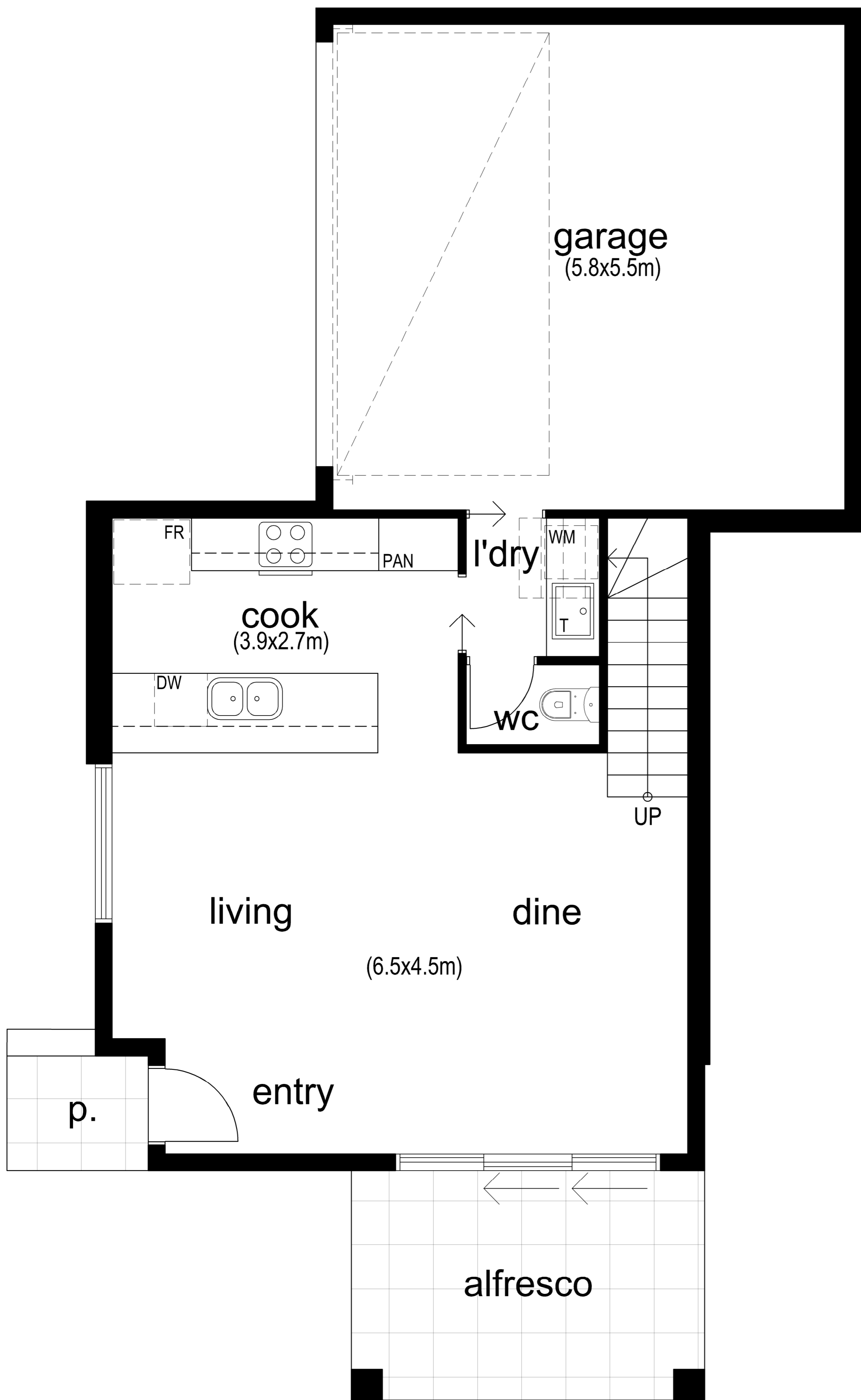
GROUND FLOOR PLAN DWELLING 1
