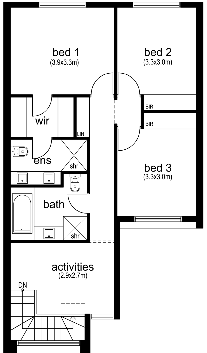
UPPER FLOOR PLAN DWELLING 5
